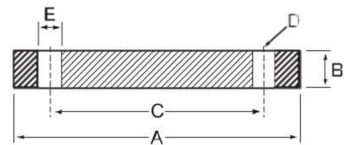
BLIND
