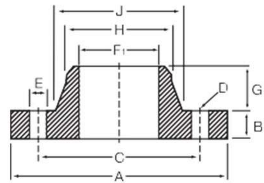
WELDING NECK
