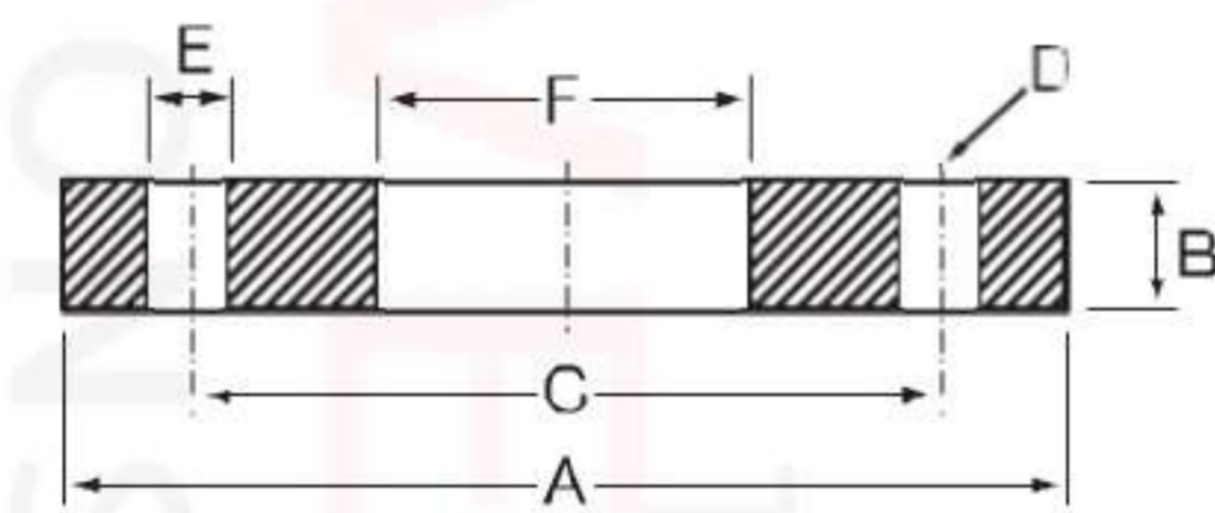
SLIP-ON WELDING
