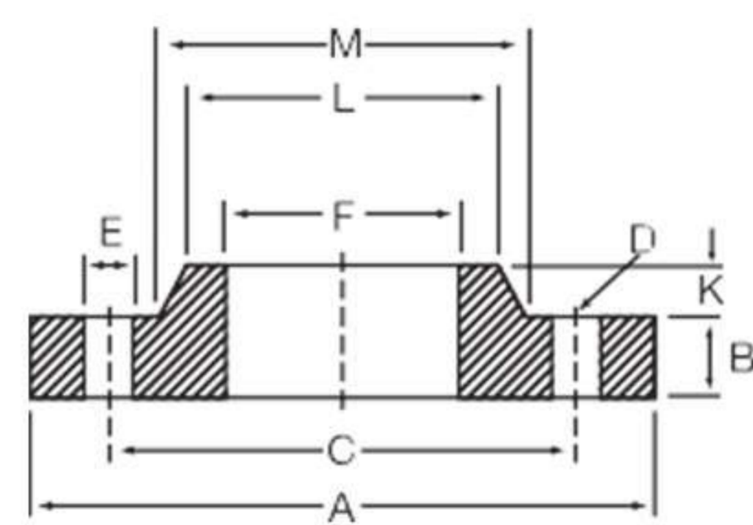
BOSSED
